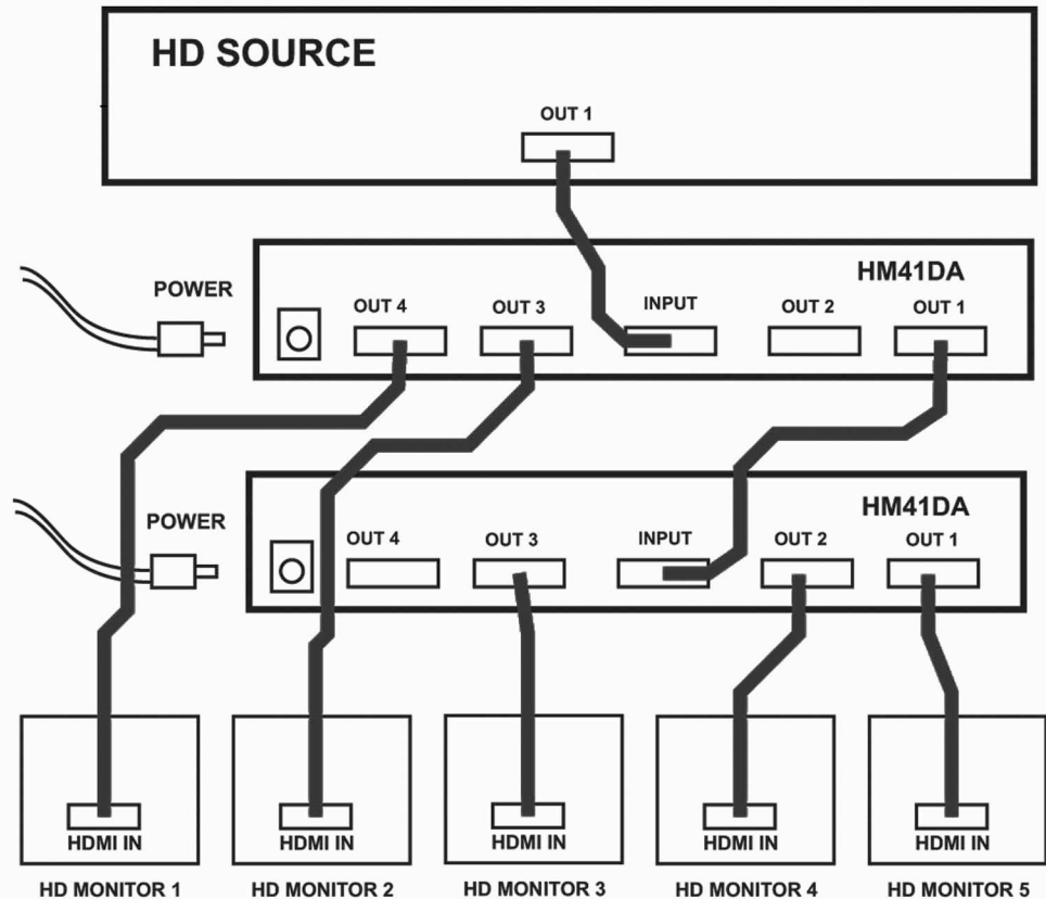
(This diagram is of the typical HM41DA connection.)
